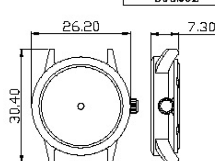
Mov't 2035 material: SS S9329L
