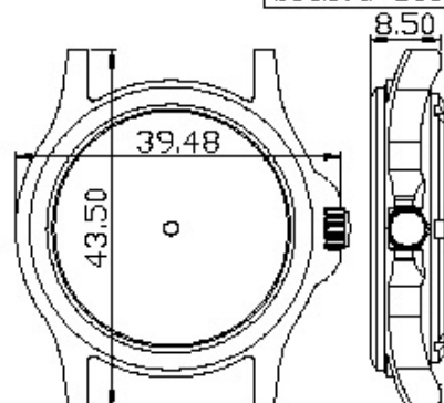
Mov't 1L12 material: SS S9327G-S93832G
