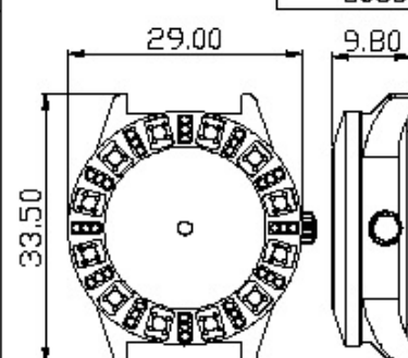
Mov't 6P89 material: SS S9330L
