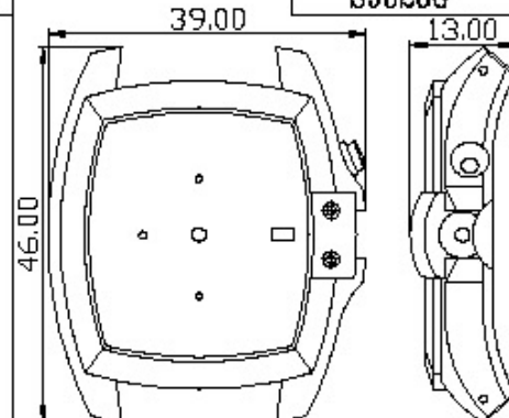
Mov't 6P89 material: SS S9330L
