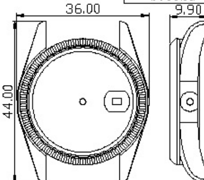
Mov't 2035 material: SS S9332G
