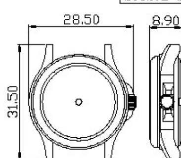
Mov't 1M12 material: SS S9327L-S93832L
